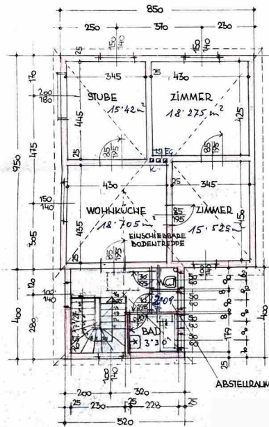
1. STOCK = 73.345 m 2
